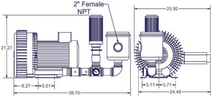
Kit Vacuum 2" NPT KVHRB902
