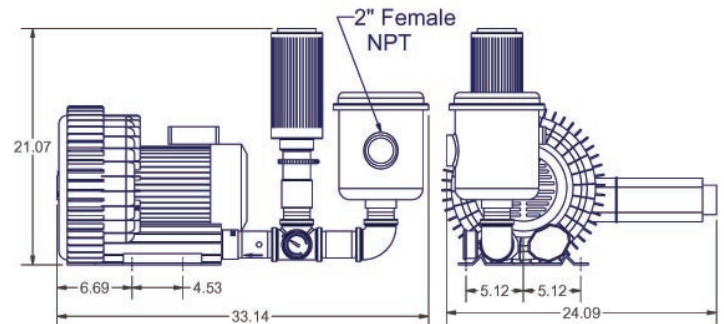
Kit Vacuum 2" NPT KVHRB502
