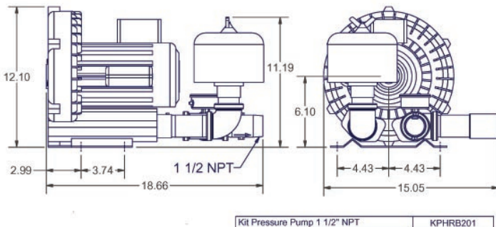
Kit Pressure Pump 1 1/2" NPT KPHRB201
