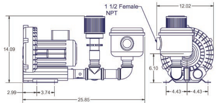
Kit Vacuum Pump 1 1/2" NPT KVHRB201
